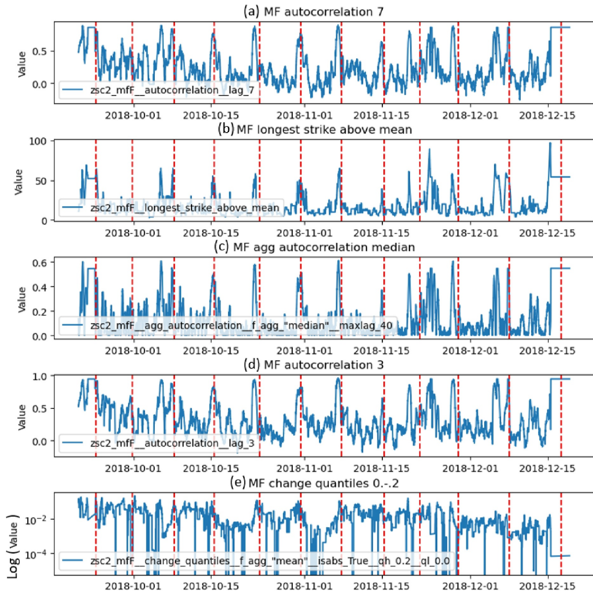
Figure 8. Time series of five key features derived from the medium frequency seismic data over the test period (out-of-sample), spanning from September 2018 to December 2018. These features were identified as significant during model training based on their importance weights in the random forest classifier, demonstrating some explainable AI (xAI) aspect of our approach. From top to bottom: Autocorrelation at lag 7, Longest strike above mean, Median of aggregated autocorrelation, Autocorrelation at lag 3, Change in quantiles (0–0.2). Each subplot shows the evolution of a specific feature over time. Vertical dashed red lines indicate eruption times. Note the varying scales on the y-axes, reflecting the different units and ranges of each feature. The plots reveal discernible increases and peaks in autocorrelation features preceding many eruption events, highlighting their potential as eruption precursors. These features, among numerous others, contribute to the model's forecasting capability, even with out-of-sample data. Data gaps are present around the first and last eruptions, potentially limiting pre-eruptive information for these events.
