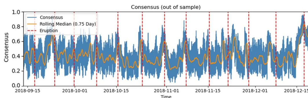
Figure 4. The blue line shows the consensus values of the trained Machine Learning model over the test period (out-of-sample). The orange line shows a rolling median of 0.75 days of the consensus values. The eruption times are marked by vertical dashed red lines.
