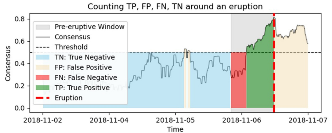
Figure 2. Performance evaluation of an eruption forecasting model for Steamboat Geyser. The graph illustrates how the consensus time series (gray line), which is the output of the eruption forecasting classifier model, can be used to quantify the model performance by setting a pre-eruptive window (gray shaded area, representing an 18-hr window) and an arbitrary threshold (dashed horizontal line). The colored areas represent: True Positives (TP, green): Model output exceeding the threshold within the pre-eruptive window; False Negatives (FN, red): Model output below the threshold within the pre-eruptive window; False Positives (FP, beige): Model output exceeding the threshold outside the pre-eruptive window, showing incorrectly forecasted eruptions; True Negatives (TN, blue): Model output below the threshold outside the pre-eruptive window, indicating correctly classified non-eruptive periods. The vertical red dashed line marks the actual eruption time. The selection of the threshold value controls the number of TP, FP, FN, and TN. In this study, to avoid selecting arbitrary thresholds when evaluating model performance, 100 thresholds equally distributed between 0 and 1 are tested, each of which generates a point on the Receiver Operator Curves curve (Section 2.2.4).
