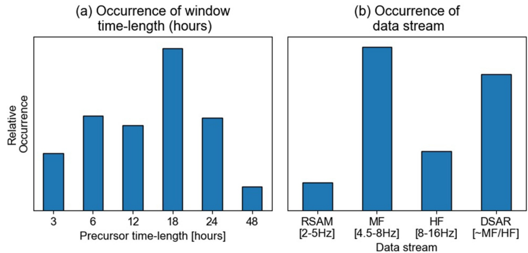
Figure 3. Evaluation of the efficacy of template-based methods through p -value analyses of correlation coefficient time series. This analysis helps identify feature families that perform better in distinguishing pre-eruptive data. For templates showing the 5% lowest p -values, adjusted for false discovery rate, we further investigated which precursor time-lengths (a) and data streams (b) exhibited the highest discriminability. Using an FDR-adjusted 5th quantile highlights the most useful ones. The 18-hr time window (a) provides the best discrimination of pre-eruptive behavior, although windows between 6 and 24 hr are also useful. Additionally, there is variability in the relative importance of different data streams during the pre-eruptive period, with medium frequency and displacement seismic amplitude ratio featuring most frequently.
