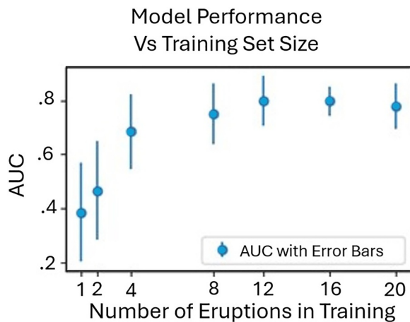
Figure 7. Model performance (AUC) as a function of the number of eruptions used for training, illustrating a “stress test” on training-set size. Each point represents the average AUC across five randomized selections (drawn from 21 events), and the error bars denote standard deviations among those five runs. All models are evaluated on the same out-of-sample data (10 eruptions). Performance steadily increases and stabilizes above approximately 9 eruptions in the training set, indicating that a moderate number of well-labeled eruptions is sufficient for robust out-of-sample generalization.
