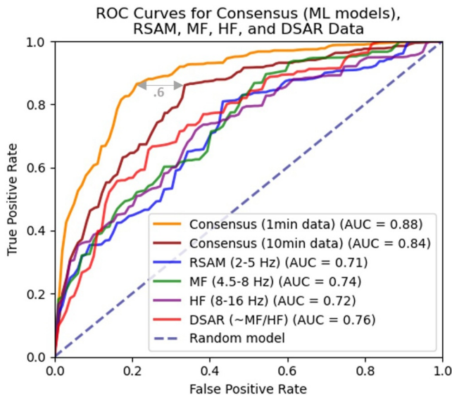
Figure 6. Receiver Operator Curves (ROC) curves (Receiver Operating Characteristic) and AUC (Area Under the Curve) illustrating the performance of the Machine Learning (ML) consensus models (1 and 10 min data) and various seismic indicators over the analyzed period. The orange curve represents the ML consensus model using 1-min data (AUC = 0.88), and the brown curve represents the ML consensus model using 10-min data (AUC = 0.84). The blue, green, purple, and red curves represent RSAM (2–5 Hz), medium frequency (4.5–8 Hz), high frequency (HF) (8–16 Hz), and displacement seismic amplitude ratio (~MF/HF) models, respectively. The diagonal dashed line represents a reference model with zero predictive power. Each point on the ROC curves corresponds to a different classification threshold. The higher AUC of the consensus models, particularly the 1-min data, indicates their superior discriminative ability compared to the other seismic indicators. As a reference, the location of the 0.6 threshold is shown (light gray). A colorblind-friendly version of this figure is provided in Figure S9 in Supporting Information S1.
